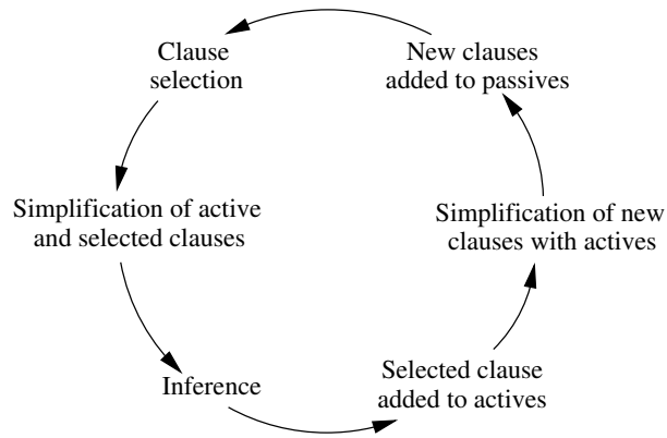
Figure 1: given-clause algorithm
