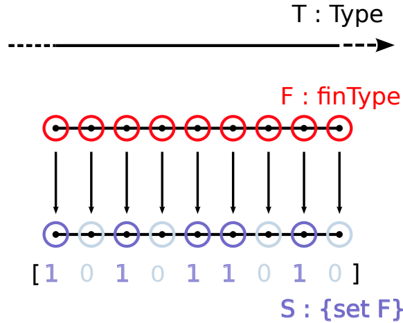
Fig. 3. Finite sets as masks on finite types
